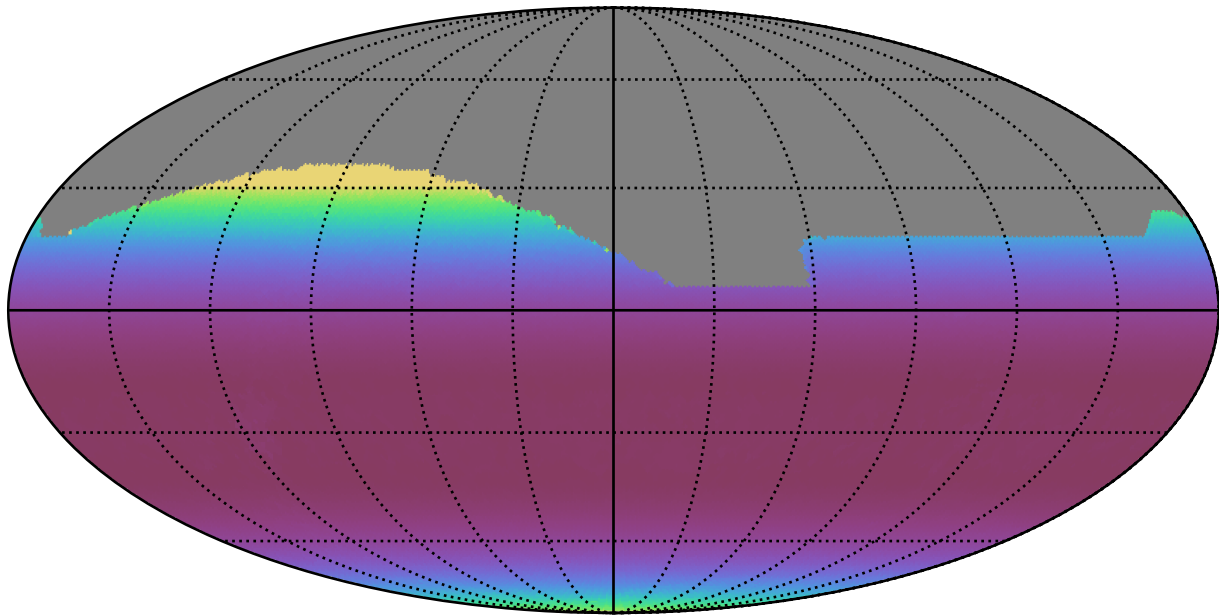
weather_cloudso10v3.4_10yrs All sky all bands: Min airmass
