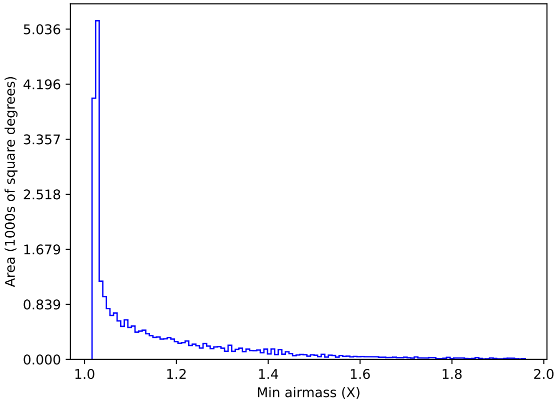
weather_cloudso10v3.4_10yrs All sky all bands: Min airmass
