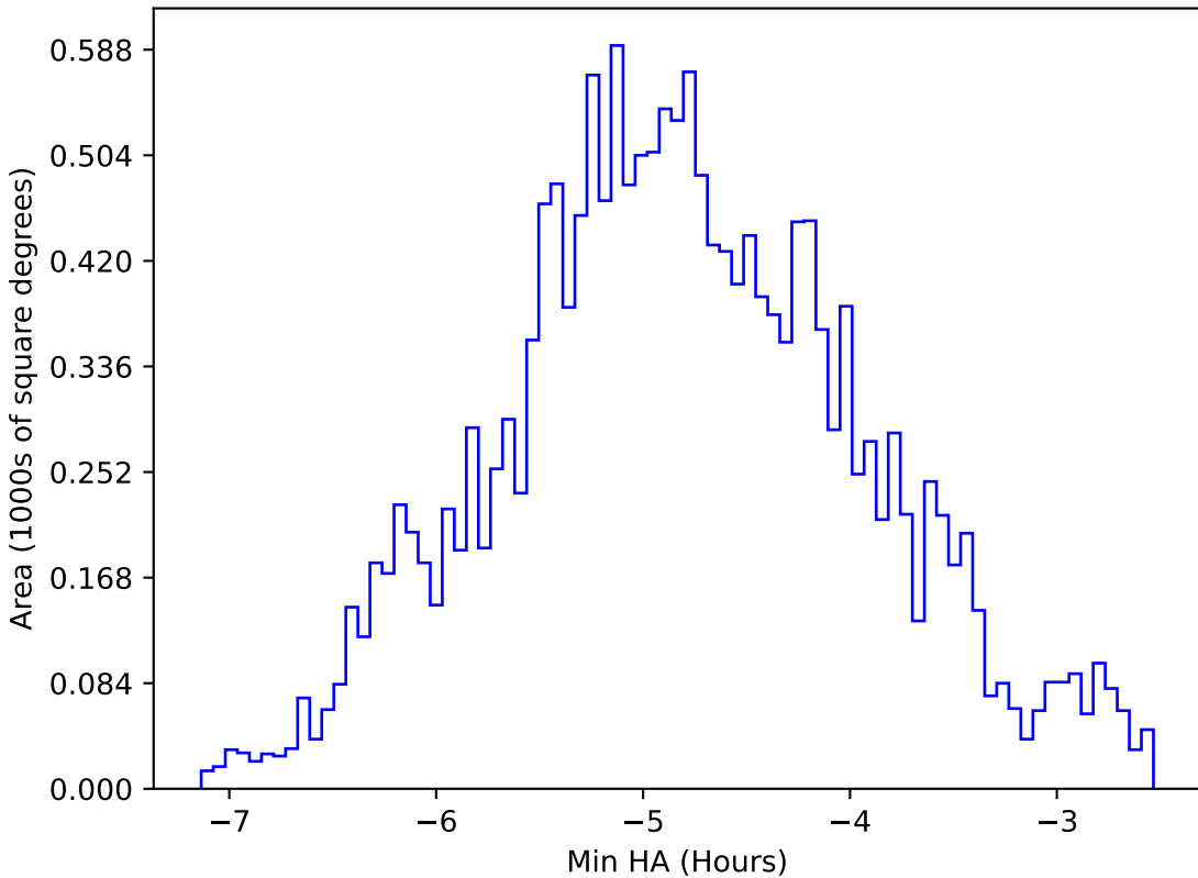
weather_cloudso10v3.4_10yrs WFD all bands: Min HA
