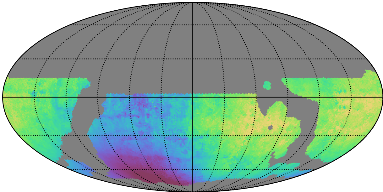
weather_cloudso10v3.4_10yrs WFD z band: Median solarElong
