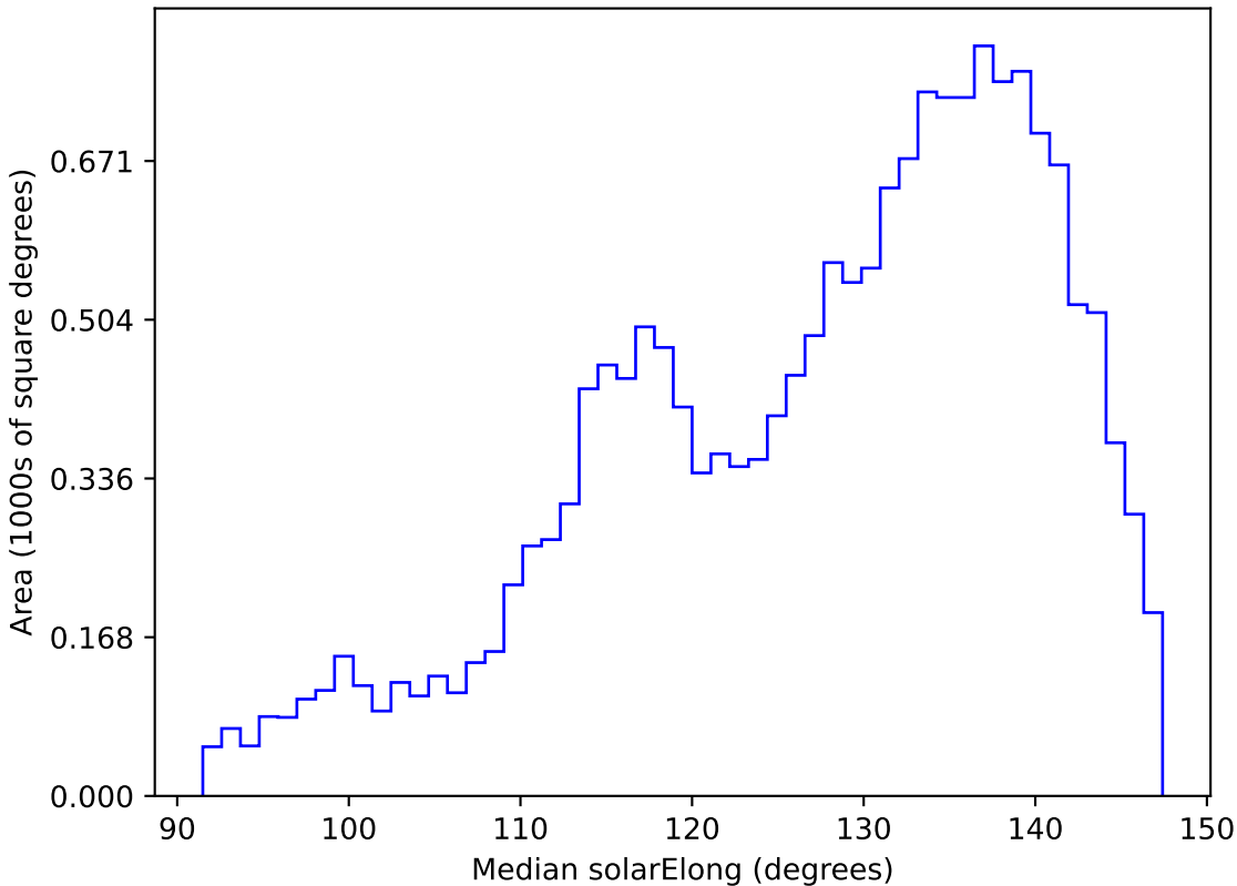
weather_cloudso10v3.4_10yrs WFD z band: Median solarElong
