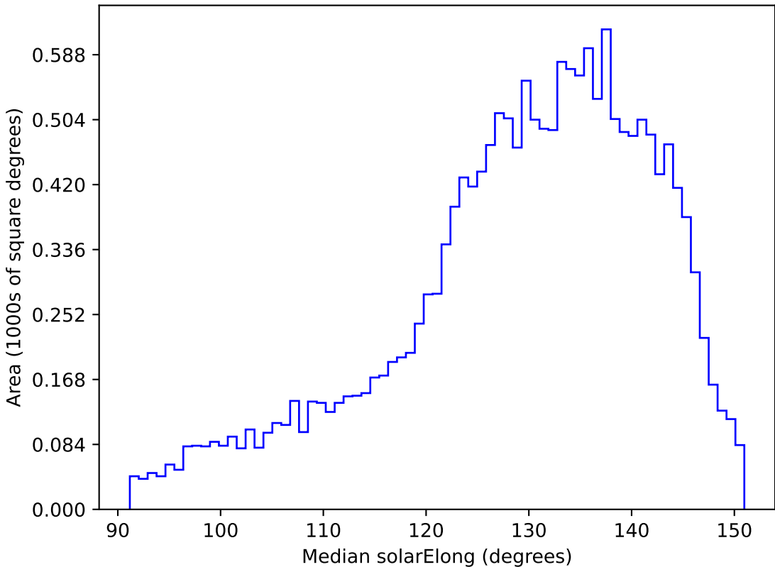
weather_cloudso10v3.4_10yrs WFD y band: Median solarElong
