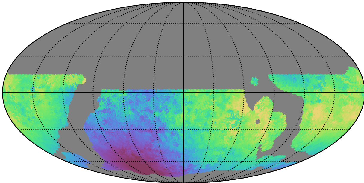
weather_cloudso10v3.4_10yrs WFD u band: Median solarElong
