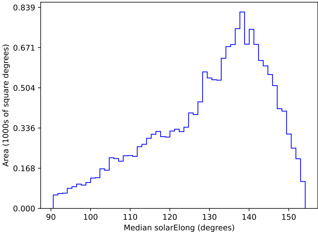
weather_cloudso10v3.4_10yrs WFD u band: Median solarElong
