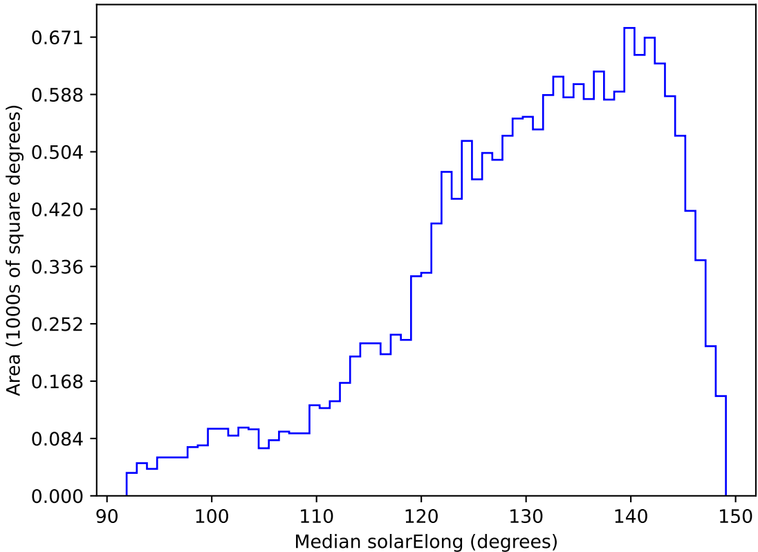
weather_cloudso10v3.4_10yrs WFD r band: Median solarElong
