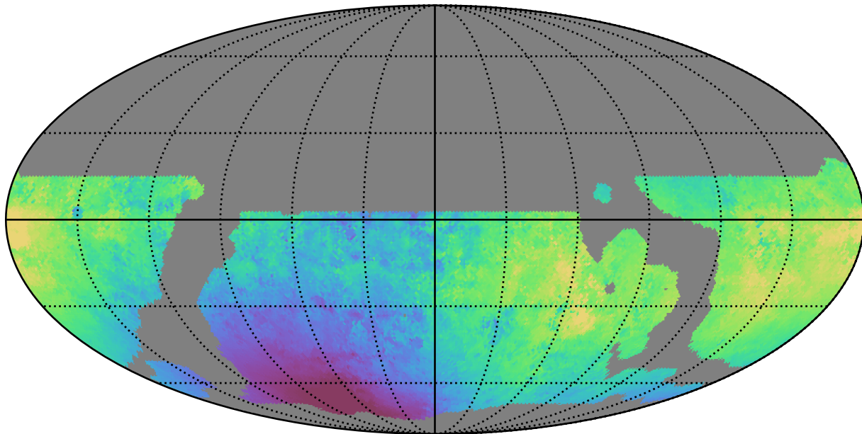
weather_cloudso10v3.4_10yrs WFD g band: Median solarElong
