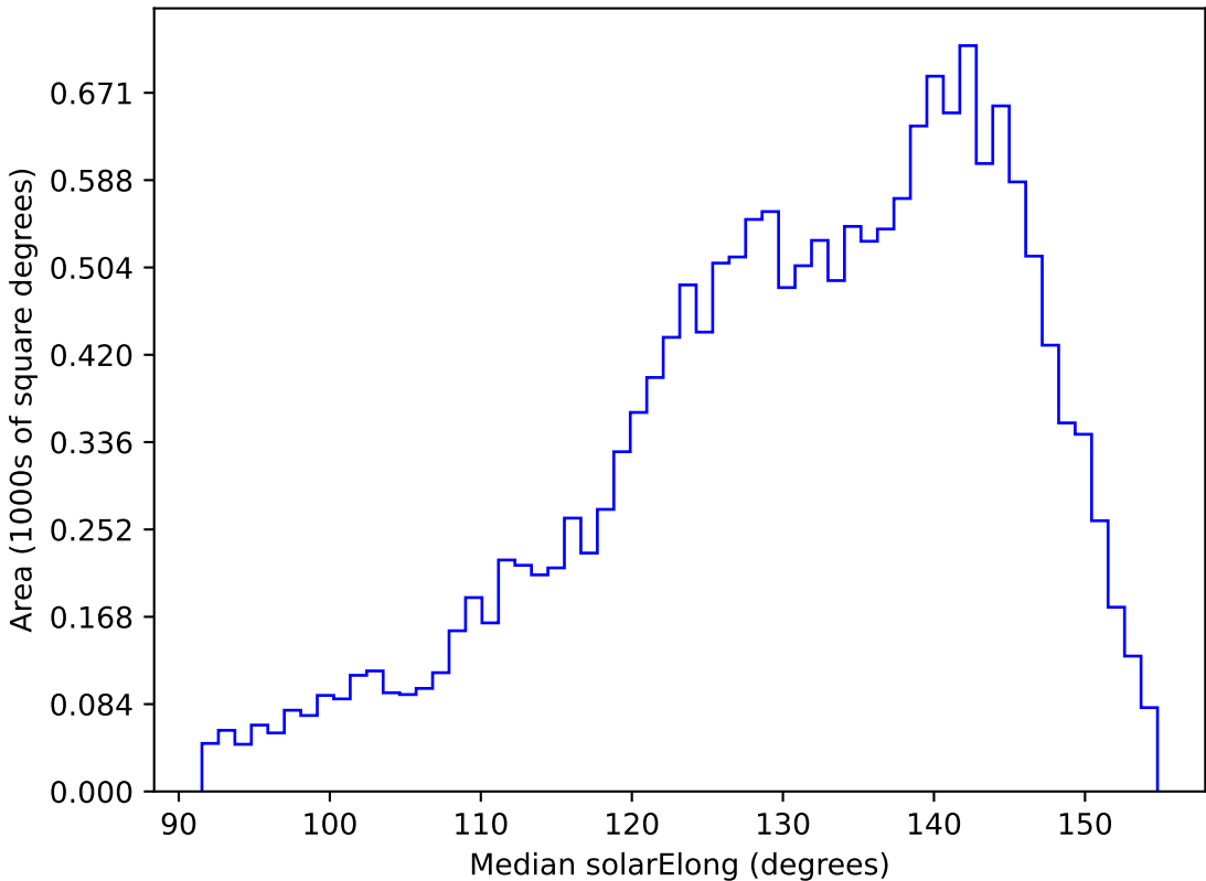
weather_cloudso10v3.4_10yrs WFD g band: Median solarElong
