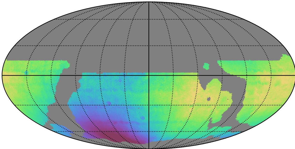
weather_cloudso10v3.4_10yrs WFD all bands: Median solarElong
