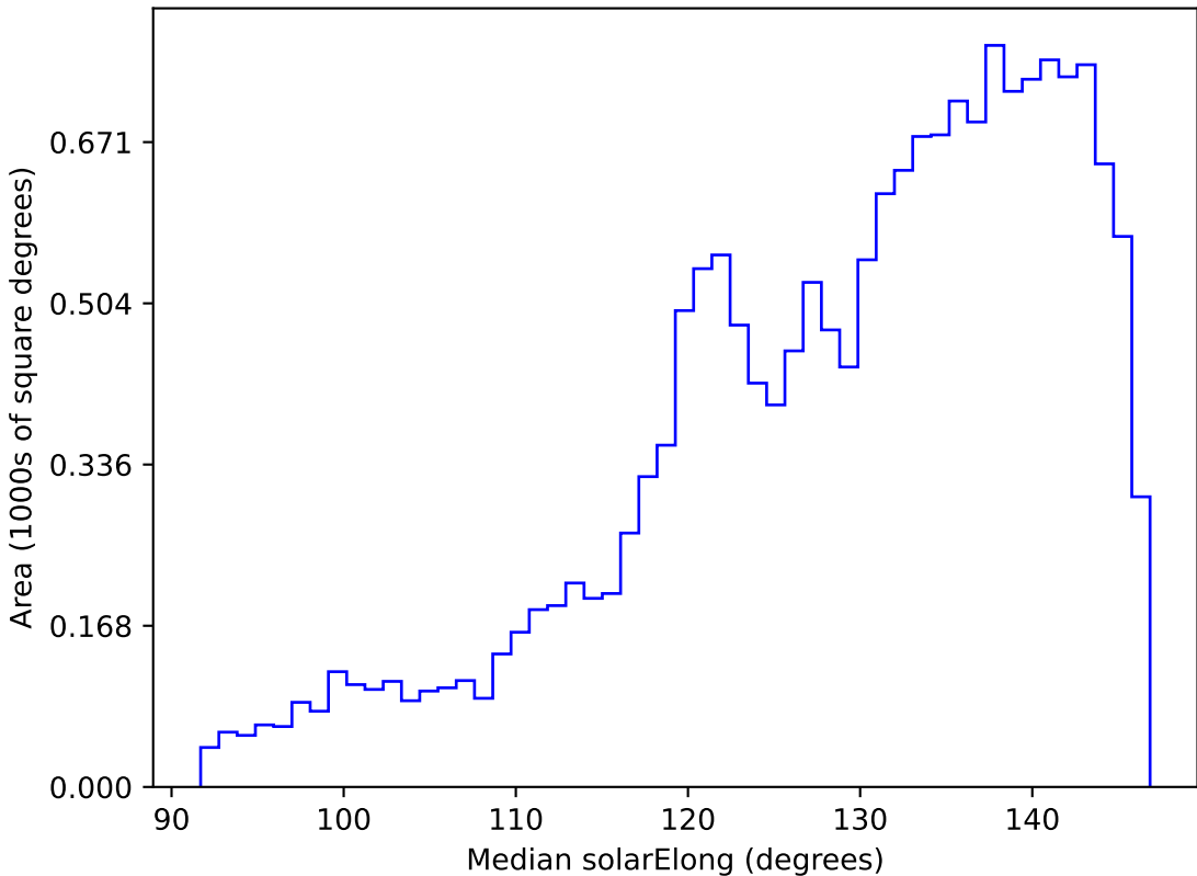
weather_cloudso10v3.4_10yrs WFD all bands: Median solarElong
