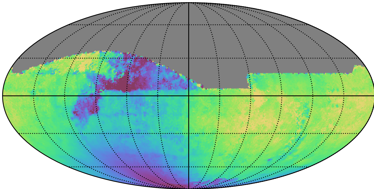
weather_cloudso10v3.4_10yrs All sky z band: Median solarElong
