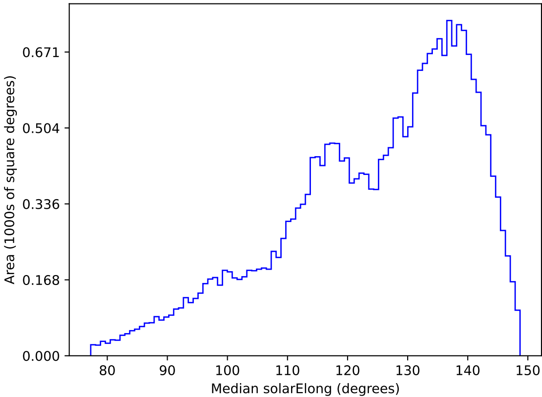
weather_cloudso10v3.4_10yrs All sky z band: Median solarElong
