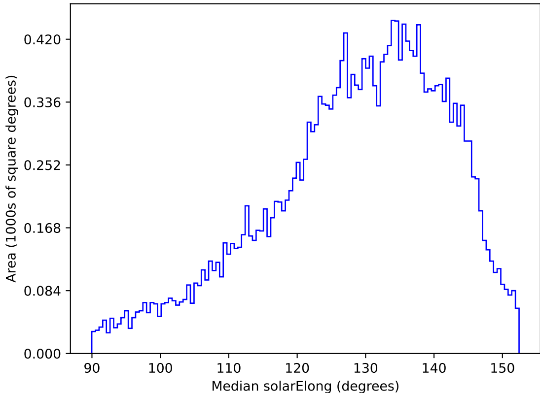
weather_cloudso10v3.4_10yrs All sky y band: Median solarElong
