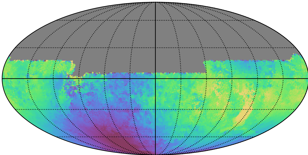
weather_cloudso10v3.4_10yrs All sky u band: Median solarElong
