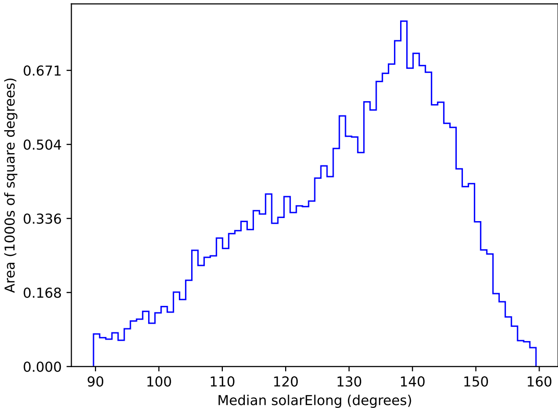
weather_cloudso10v3.4_10yrs All sky u band: Median solarElong
