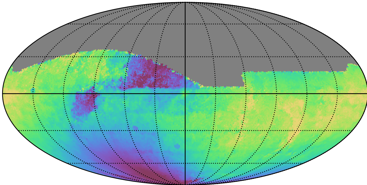
weather_cloudso10v3.4_10yrs All sky r band: Median solarElong
