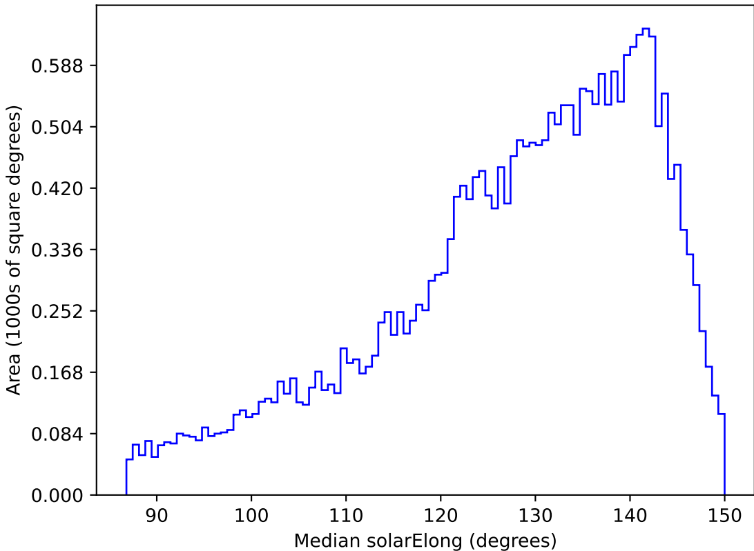
weather_cloudso10v3.4_10yrs All sky r band: Median solarElong
