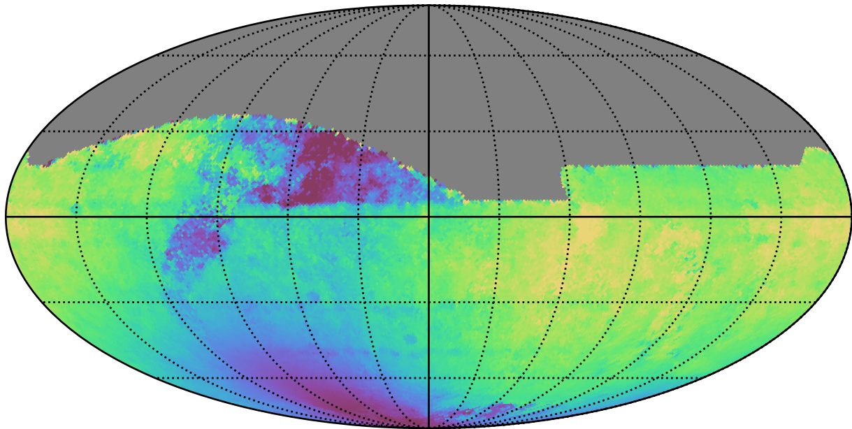
weather_cloudso10v3.4_10yrs All sky i band: Median solarElong
