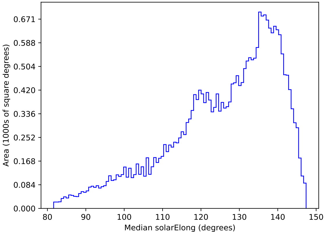
weather_cloudso10v3.4_10yrs All sky i band: Median solarElong
