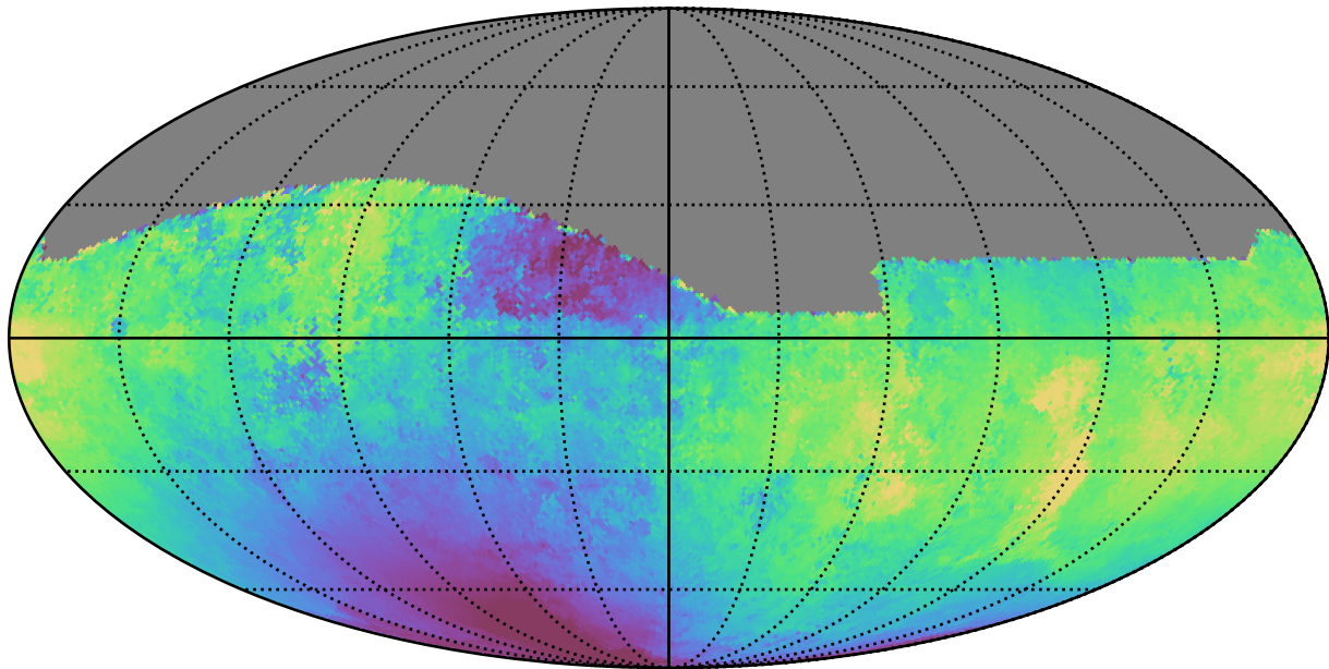
weather_cloudso10v3.4_10yrs All sky g band: Median solarElong
