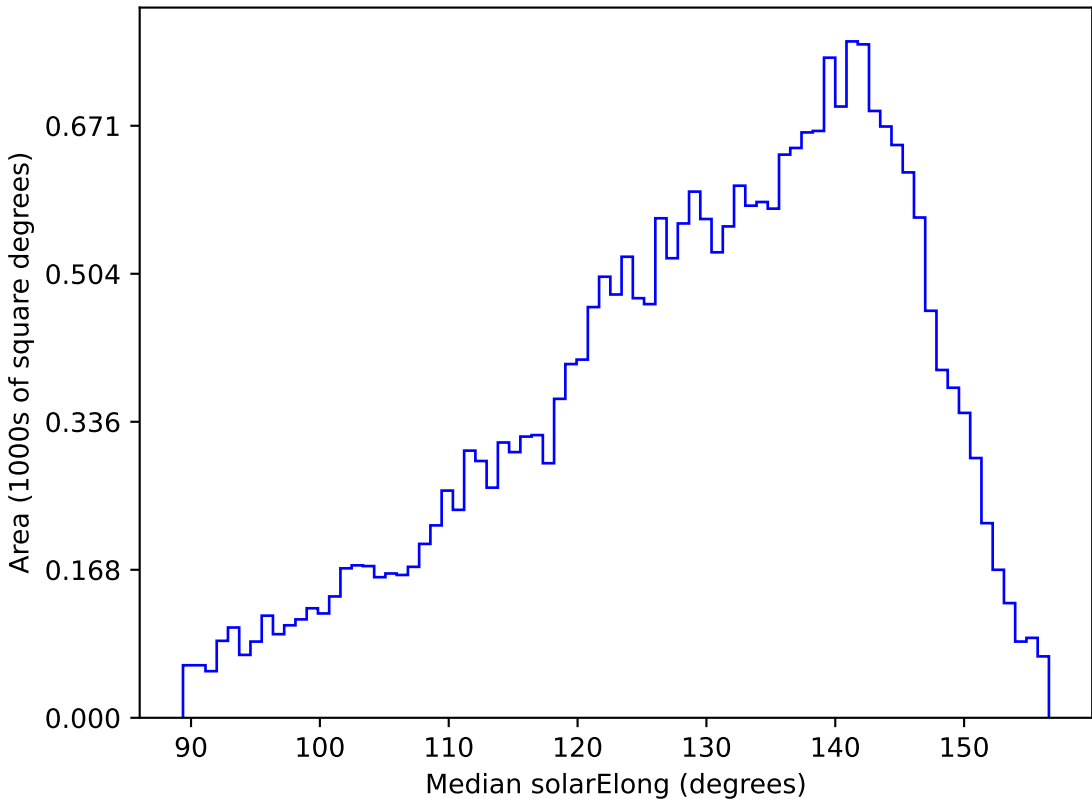
weather_cloudso10v3.4_10yrs All sky g band: Median solarElong
