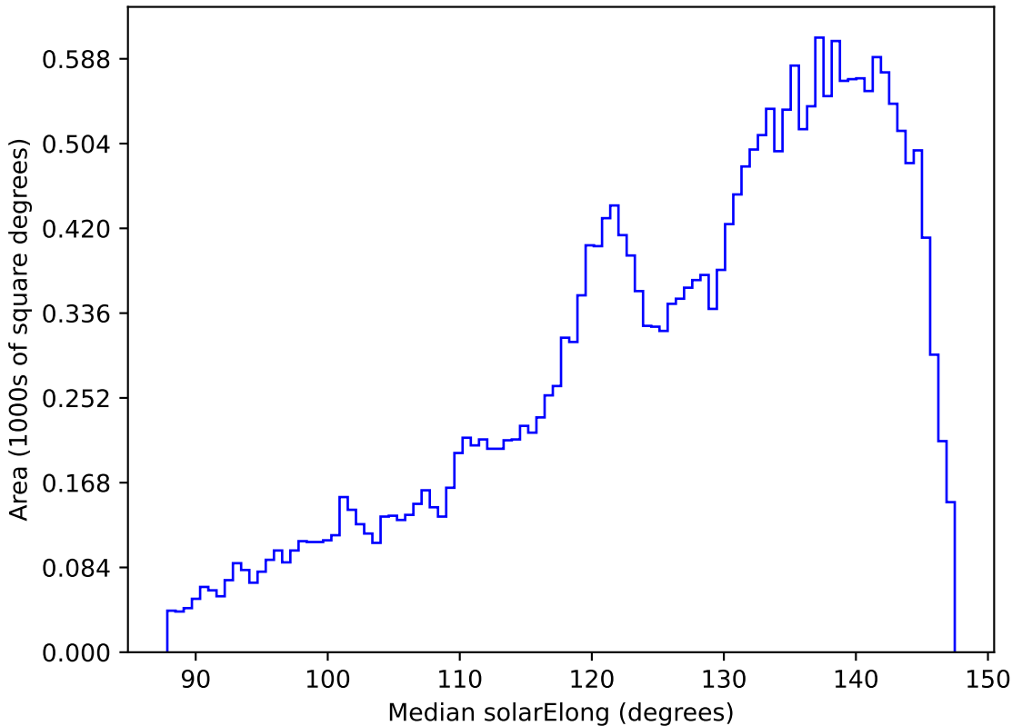
weather_cloudso10v3.4_10yrs All sky all bands: Median solarElong
