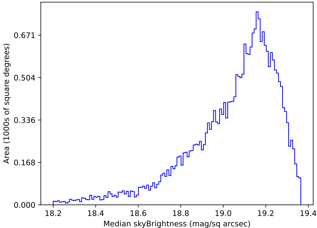
weather_cloudso10v3.4_10yrs Yr 1 z band: Median skyBrightness
