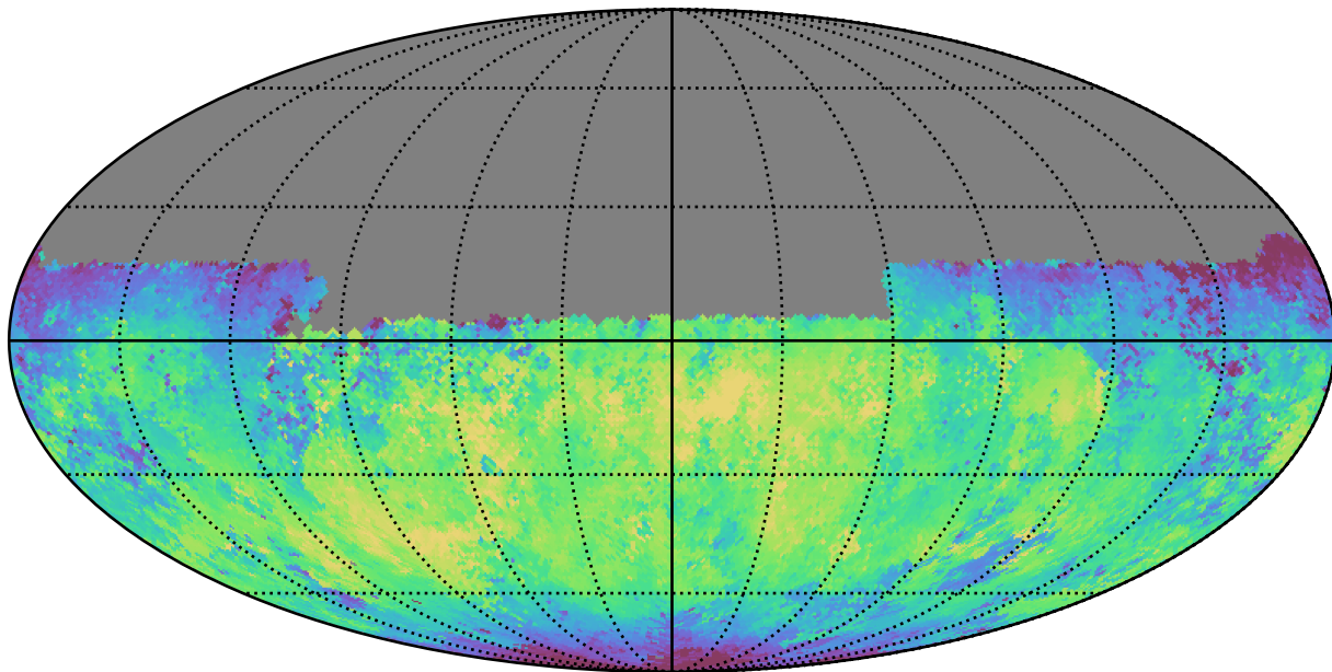
weather_cloudso10v3.4_10yrs Yr 1 y band: Median skyBrightness
