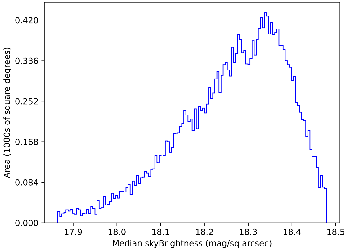
weather_cloudso10v3.4_10yrs Yr 1 y band: Median skyBrightness
