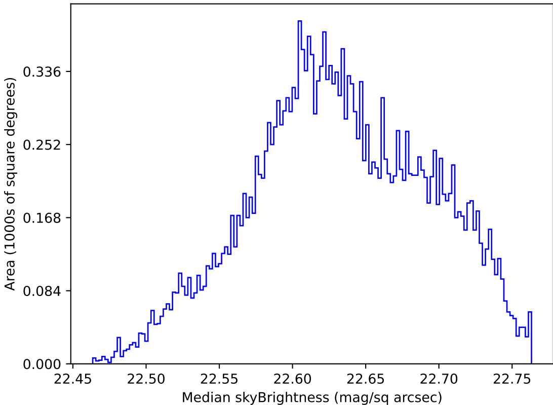
weather_cloudso10v3.4_10yrs Yr 1 u band: Median skyBrightness
