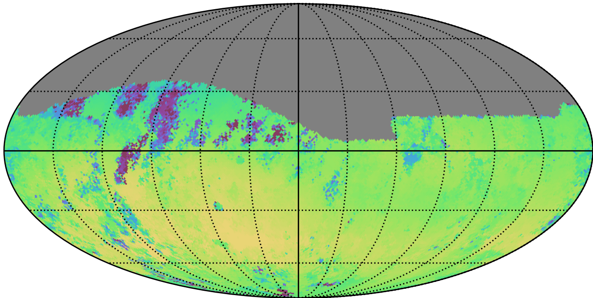
weather_cloudso10v3.4_10yrs Yr 1 r band: Median skyBrightness
