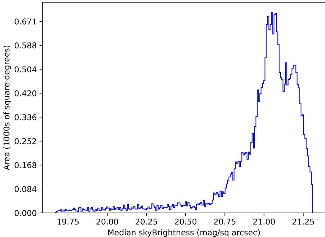
weather_cloudso10v3.4_10yrs Yr 1 r band: Median skyBrightness
