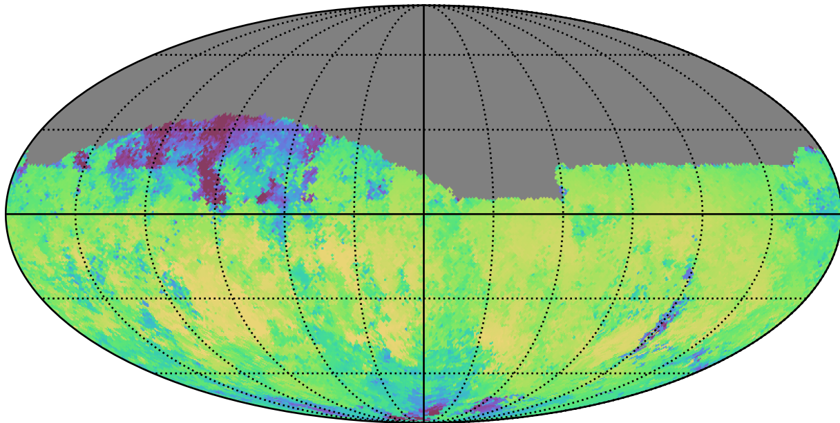
weather_cloudso10v3.4_10yrs Yr 1 i band: Median skyBrightness
