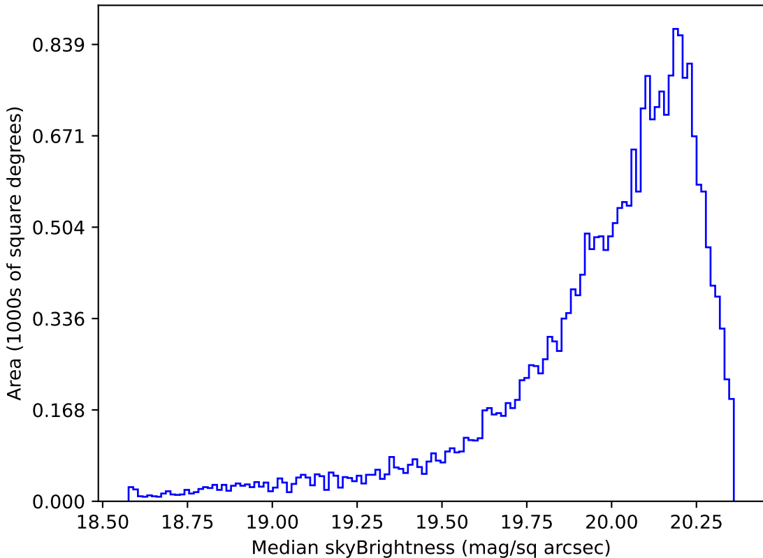
weather_cloudso10v3.4_10yrs Yr 1 i band: Median skyBrightness
