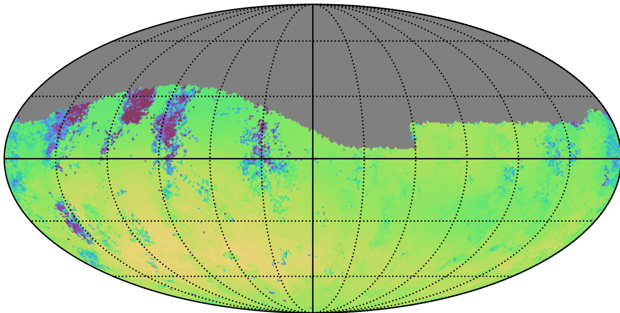
weather_cloudso10v3.4_10yrs Yr 1 g band: Median skyBrightness
