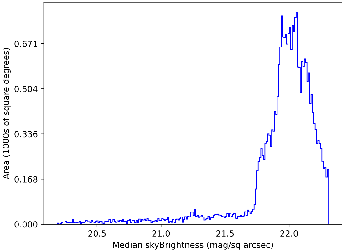
weather_cloudso10v3.4_10yrs Yr 1 g band: Median skyBrightness
