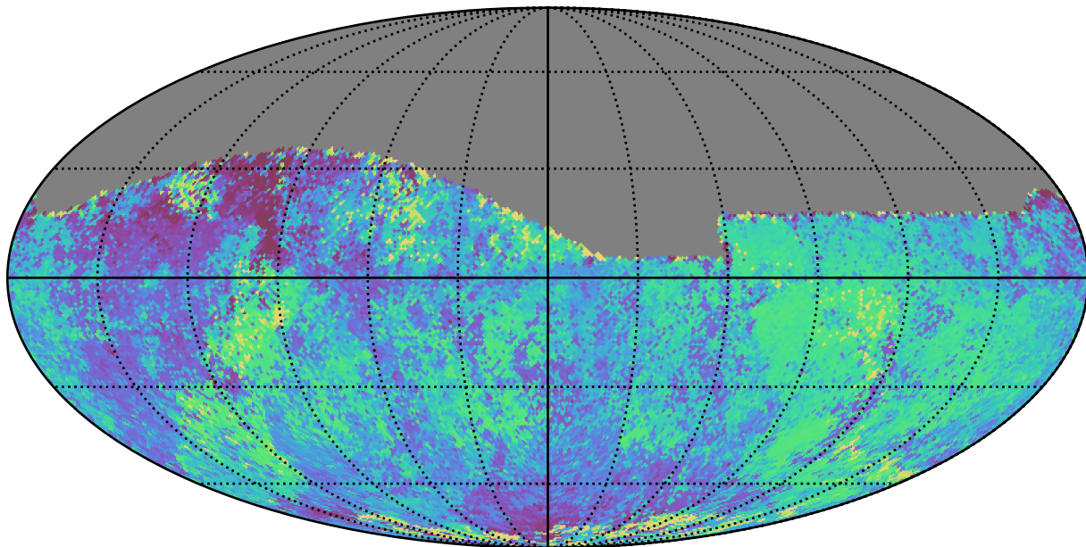
weather_cloudso10v3.4_10yrs Yr 1 all bands: Median skyBrightness
