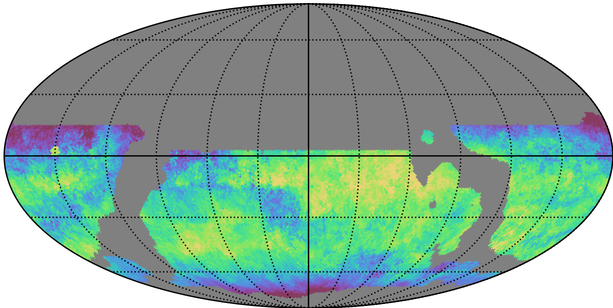
weather_cloudso10v3.4_10yrs WFD z band: Median skyBrightness
