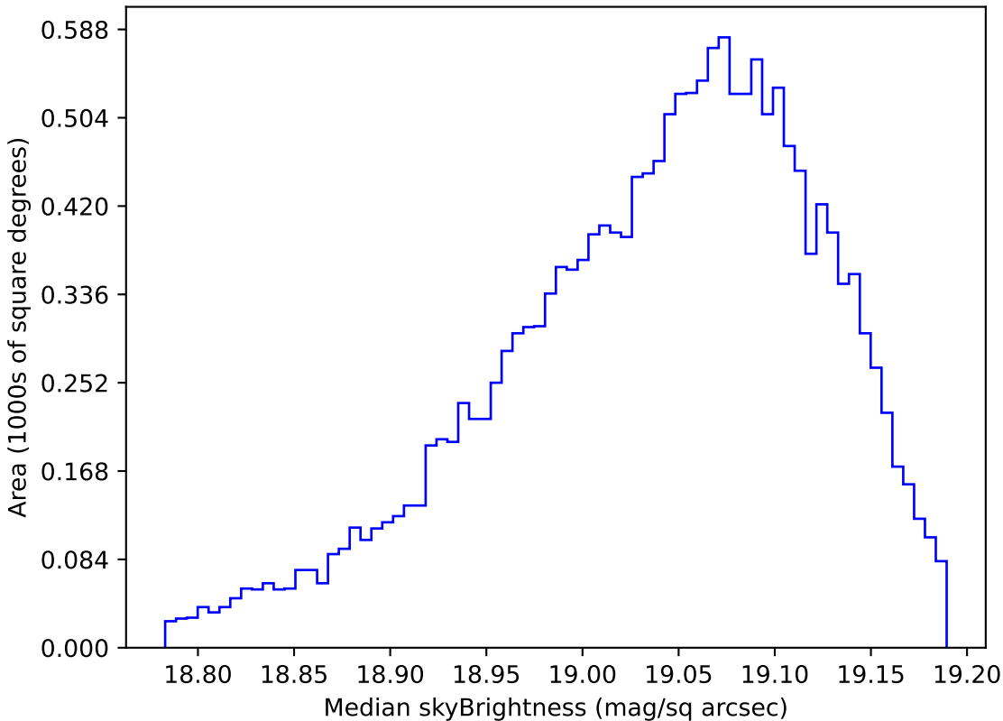
weather_cloudso10v3.4_10yrs WFD z band: Median skyBrightness
