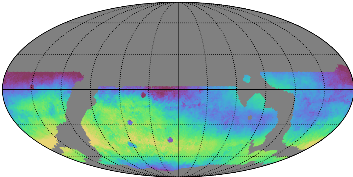
weather_cloudso10v3.4_10yrs WFD r band: Median skyBrightness
