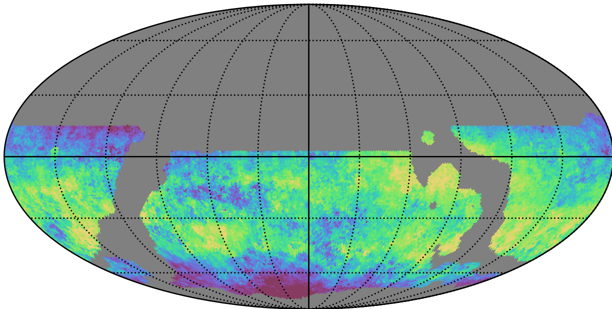
weather_cloudso10v3.4_10yrs WFD i band: Median skyBrightness
