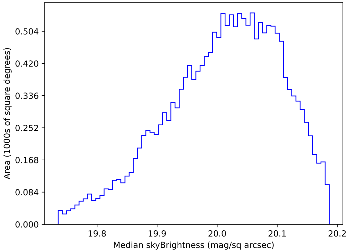
weather_cloudso10v3.4_10yrs WFD i band: Median skyBrightness
