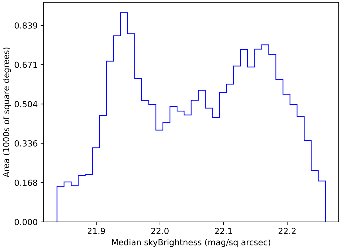
weather_cloudso10v3.4_10yrs WFD g band: Median skyBrightness
