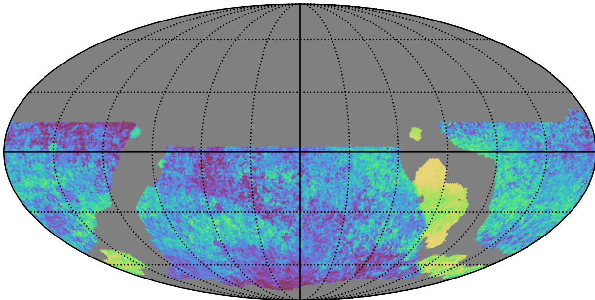
weather_cloudso10v3.4_10yrs WFD all bands: Median skyBrightness
