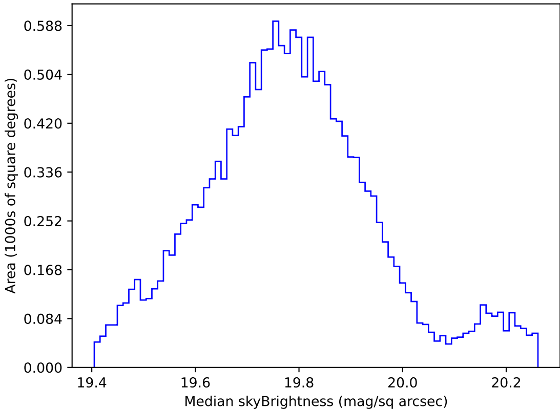
weather_cloudso10v3.4_10yrs WFD all bands: Median skyBrightness
