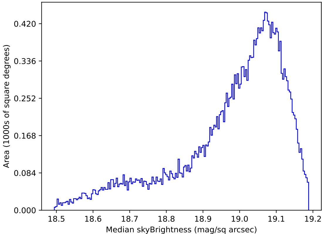
weather_cloudso10v3.4_10yrs All sky z band: Median skyBrightness
