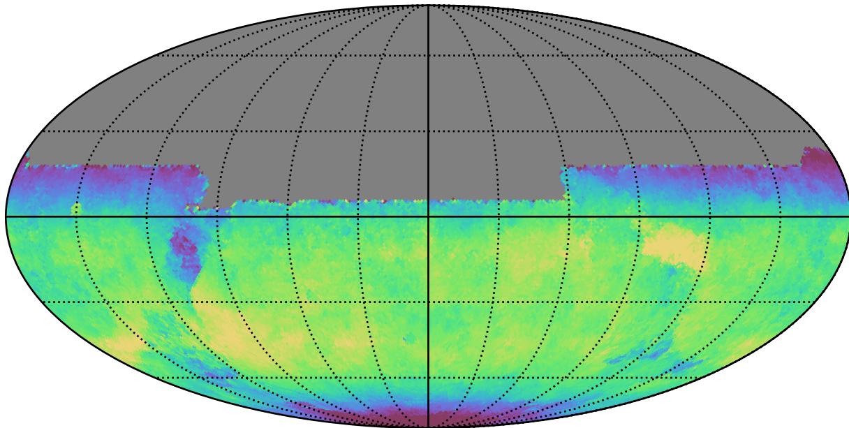
weather_cloudso10v3.4_10yrs All sky y band: Median skyBrightness
