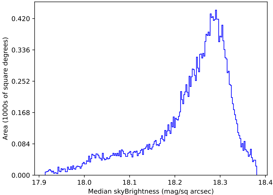
weather_cloudso10v3.4_10yrs All sky y band: Median skyBrightness
