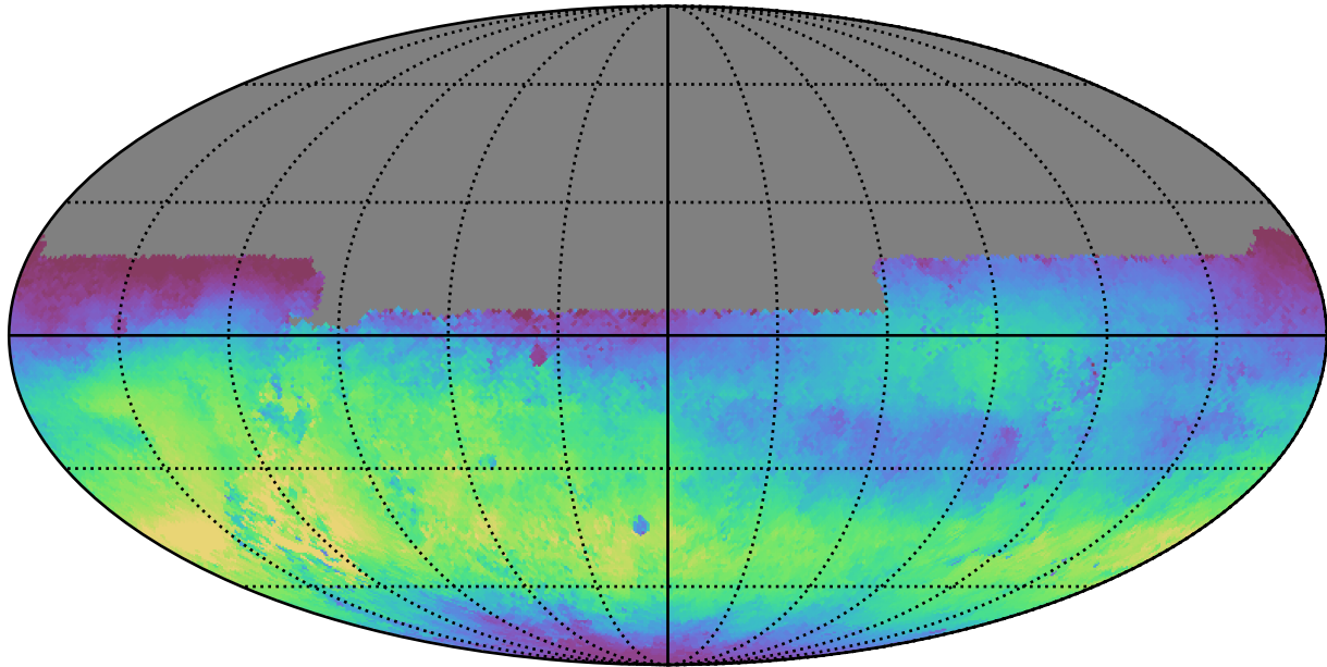
weather_cloudso10v3.4_10yrs All sky u band: Median skyBrightness
