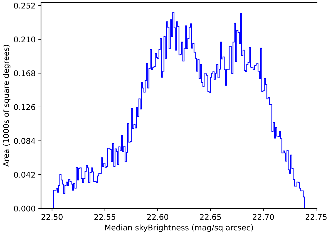
weather_cloudso10v3.4_10yrs All sky u band: Median skyBrightness
