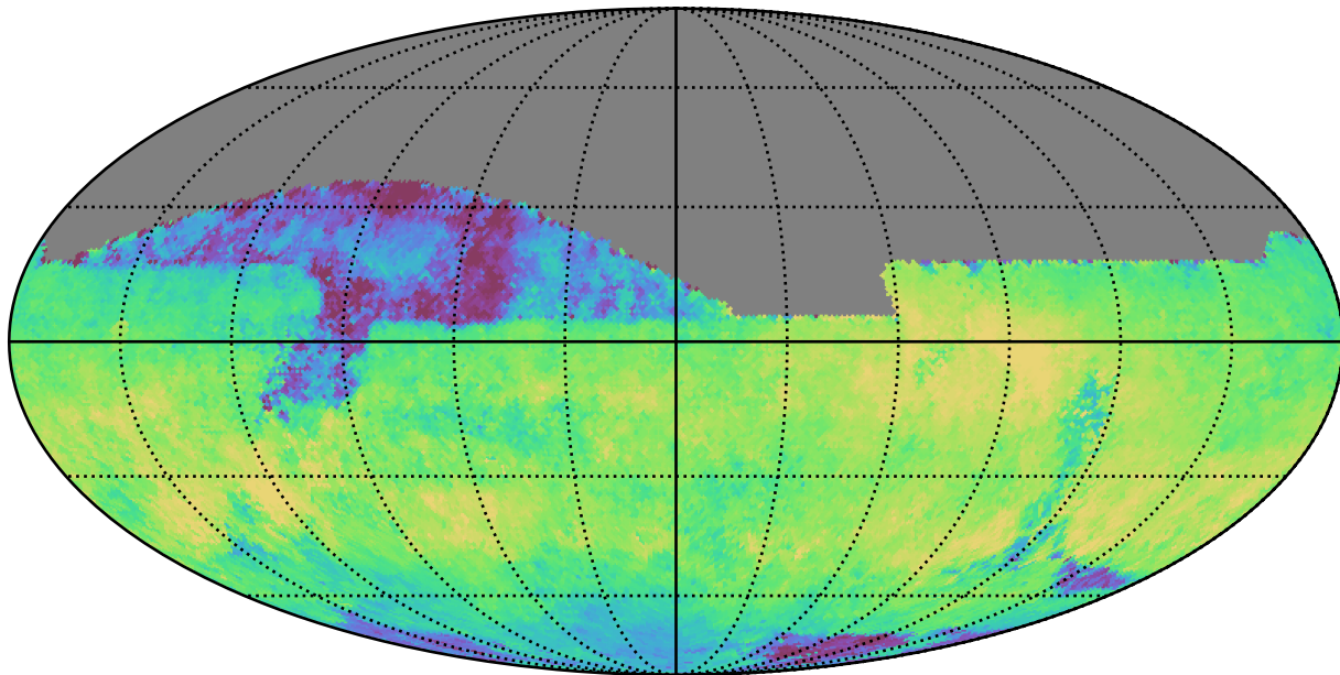
weather_cloudso10v3.4_10yrs All sky i band: Median skyBrightness
